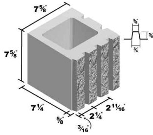
8x8x8 Half Corner Split Face 7 Taper Score
