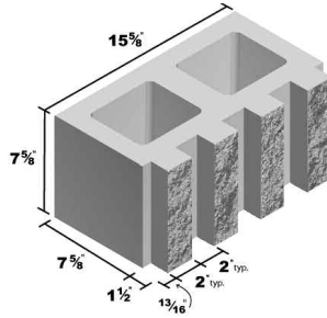
10x8x16 Standard Split Face 2" 4 Flute
