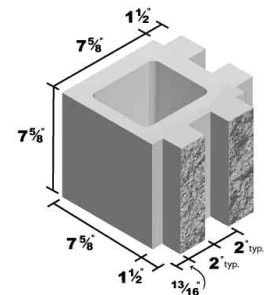
10x8x10 Half Corner Split Face 2" 4 Flute
