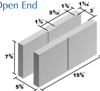
6x8x16 Double Open End Bond Beam
