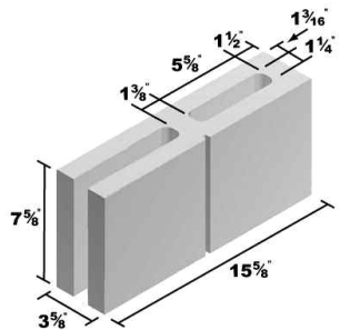
4x8x16 Open End Standard
