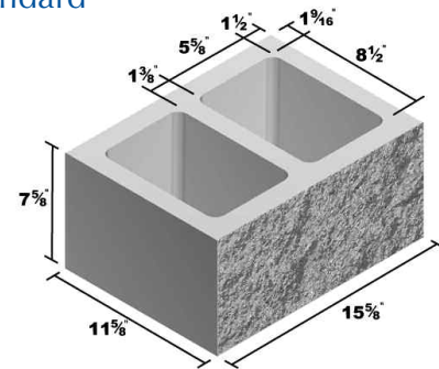
12x8x16 Standard
