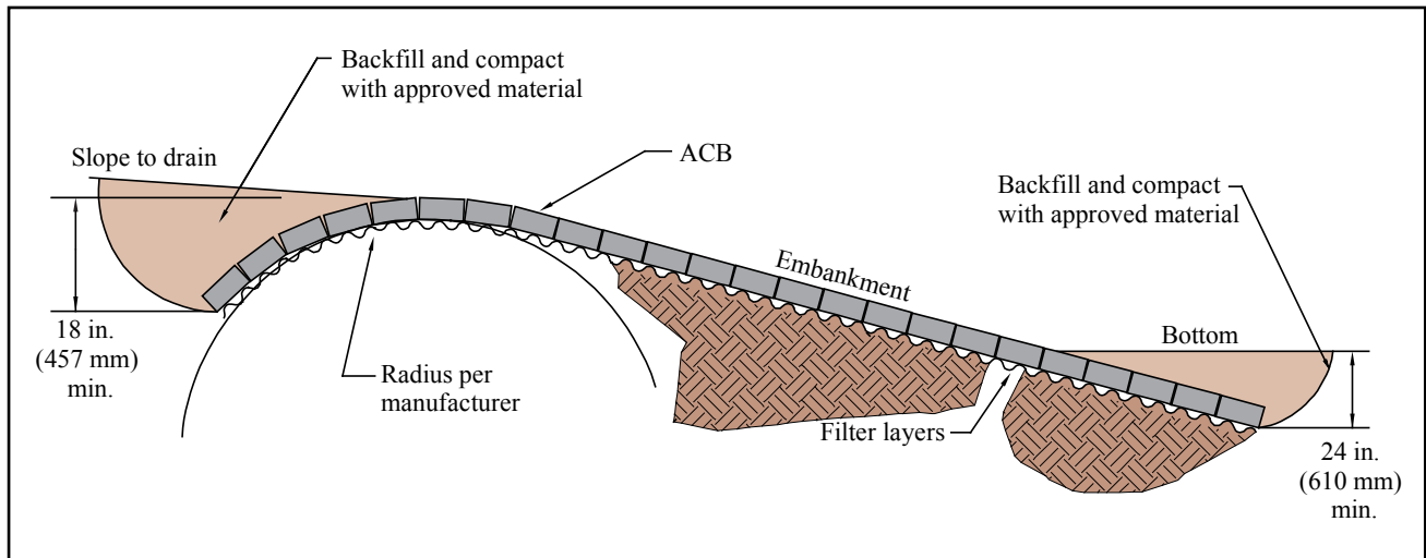
Figure 3—ACB Embankment, Typical Cross-Section
