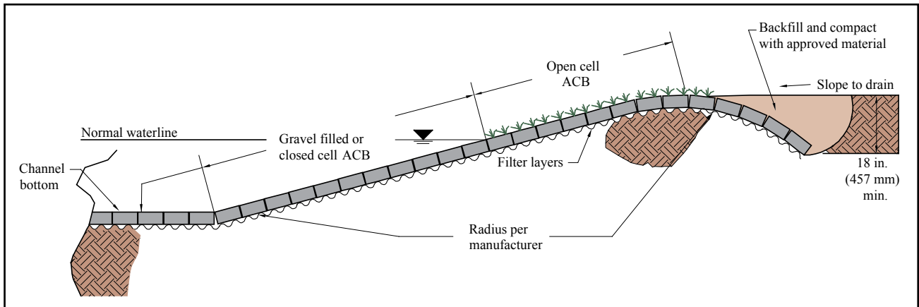
Figure 2—ACB Trapezoidal Channel Lining, Typical Cross-Section
