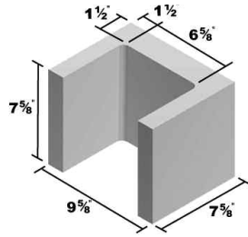
10x8x16 Double Open End Bond Beam
