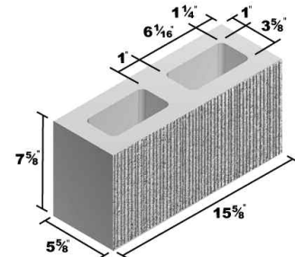
6x8x16 Standard
