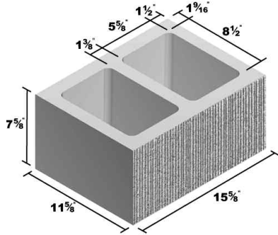
12x8x16 Standard
