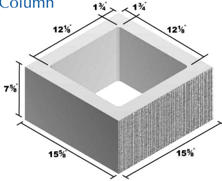
16x8x16 Column
