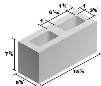
6x8x16 Standard
