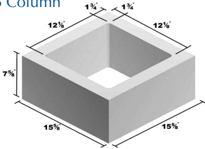
16x8x16 Column
