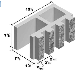
10x8x16 Open End Split Face 2" 4 Score
