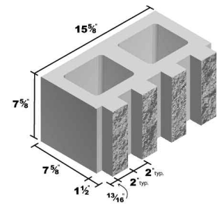
10x8x16 Standard Split Face 2" 4 Score
