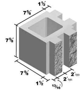
10x8x10 Half Corner Split Face 2" 4 Score
