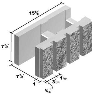
9x8x16 Open End Bond Beam Split Face 1" 4 Score
