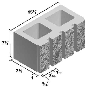
9x8x16 Standard Split Face 1" 4 Score
