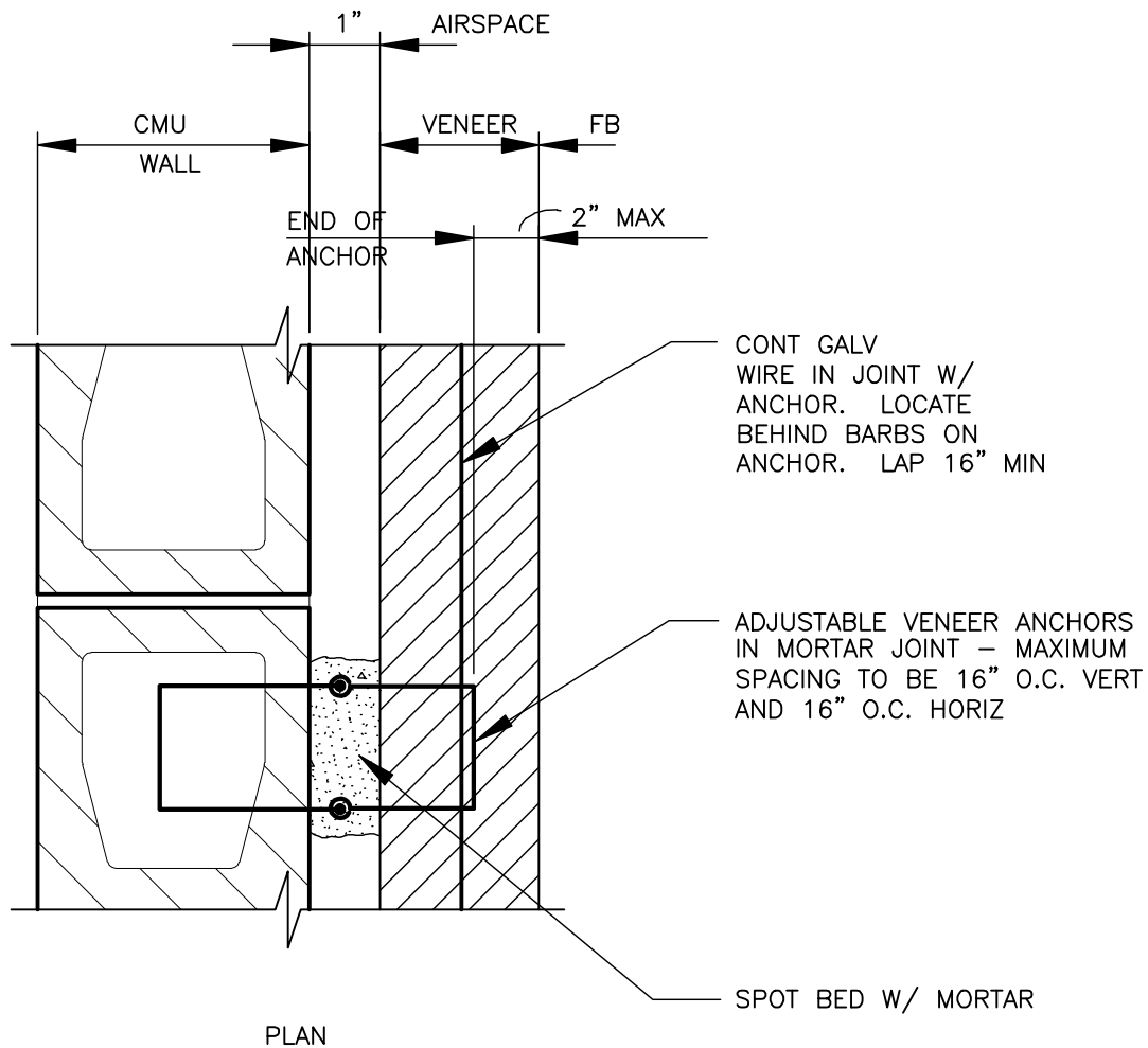
TYPICAL VENEER ANCHORAGE TO CMU
