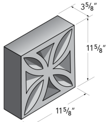
4x12x12 Viewlite 1
