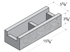
6x4x16 Solid Bottom Bond Beam
