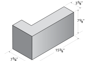
4x8x16 Spec-Brick L CNR
