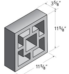
4x12x12 Viewlite 4
