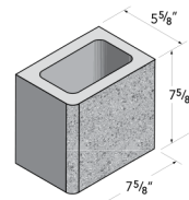
6x8x8 Single Bullnose
