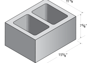
12x8x16 Spec-Brick
