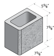
6x8x8 Double Bullnose
