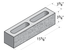
4x4x16 Standard
