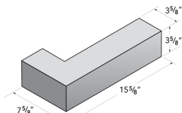
4x4x16 Spec-Brick L CNR
