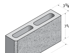
4x8x16 Single Bullnose
