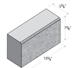
6x8x16 Solid Chamfer
