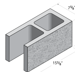
8x8x16 SCOE Block
