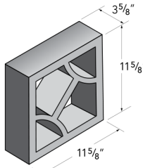
4x12x12 Viewlite 5
