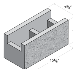
8x8x16 Solid Bottom Bond Beam
