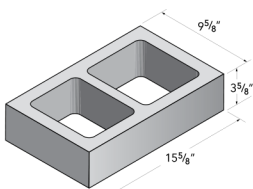
10x4x16 Spec-Brick
