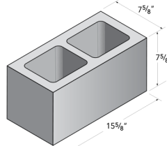
8x8x16 Spec-Brick
