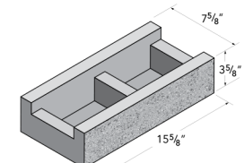
8x4x16 Solid Bottom Bond Beam
