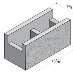
8x8x16 Bond Beam
