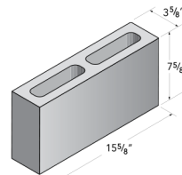
4x8x16 Spec-Brick
