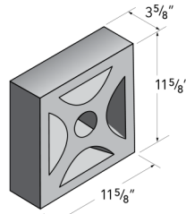
4x12x12 Viewlite 6
