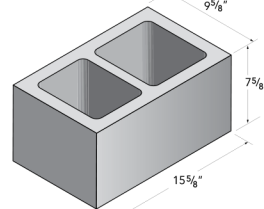
10x8x16 Spec-Brick
