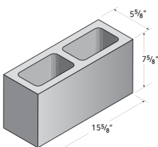
6x8x16 Spec-Brick
