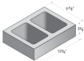
12x4x16 Spec-Brick
