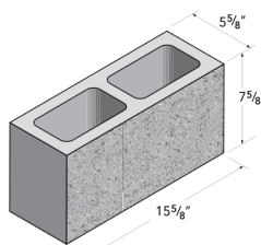
6x8x16 Standard
