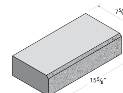
8x4x16 Solid Chamfer
