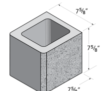
8x8x8 Double Bullnose
