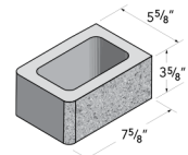
6x4x8 Double Bullnose
