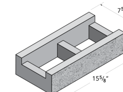
8x4x16 Bond Beam
