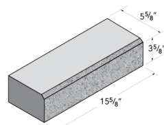
6x4x16 Solid Chamfer
