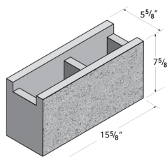
6x8x16 Solid Bottom Bond Beam
