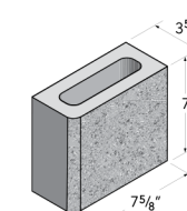
4x8x8 Single Bullnose
