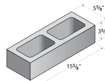
6x4x16 Spec-Brick
