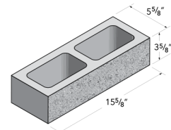
6x4x16 Standard
