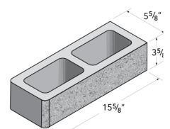
6x4x16 Double Bullnose
