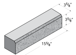
4x4x16 Solid Chamfer
