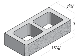
8x4x16 Single Bullnose
