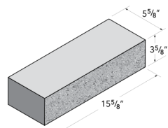
6x4x16 Solid
