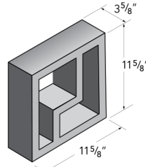
4x12x12 Viewlite 3
