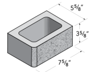
6x4x8 Single Bullnose
