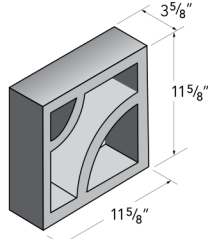
4x12x12 Viewlite 2
