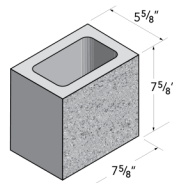
6x8x8 Standard
