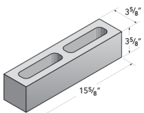
4x4x16 Spec-Brick
