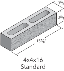
4x4x16 Standard
