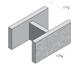
12x8x16 DOE Block
