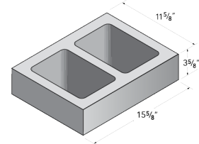
12x4x16 Spec-Brick
