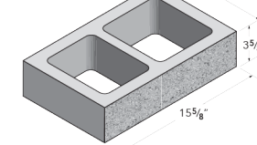
10x4x16 Standard
