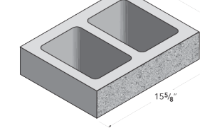
12x4x16 Standard
