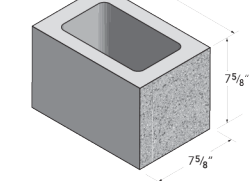
12x8x8 Standard
