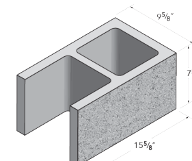
10x8x16 SCOE Block
