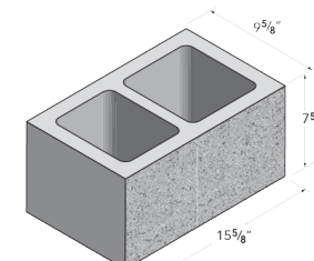
10x8x16 Standard
