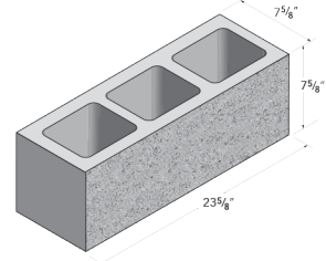
8x8x24 Standard
