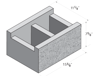
12x8x16 Bond Beam
