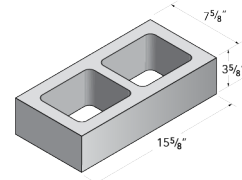
8x4x16 Spec-Brick
