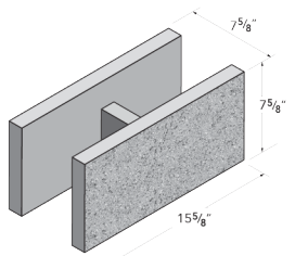
8x8x16 DOE Block
