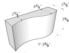
Abri Serpentine
