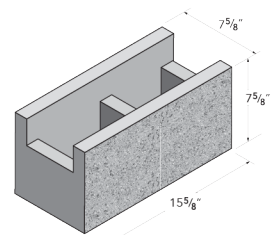
8x8x16 Bond Beam
