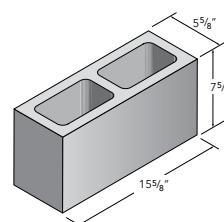
6x8x16 Spec-Brick
