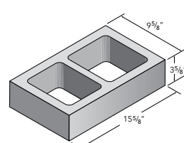
10x4x16 Spec-Brick
