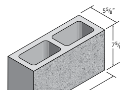
6x8x16 Standard
