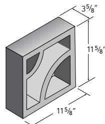
4x12x12 Viewlite 2
