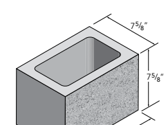
8x8x12 Standard
