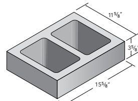
12x4x16 Spec-Brick
