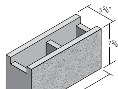
6x8x16 Bond Beam
