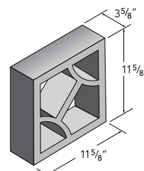
4x12x12 Viewlite 5
