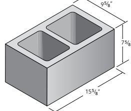
10x8x16 Spec-Brick
