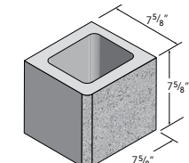
8x8x8 Single Bullnose
