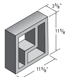
4x12x12 Viewlite 3
