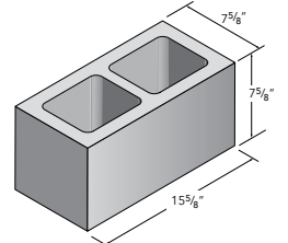
8x8x16 Spec-Brick
