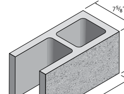
8x8x16 SCOE Block
