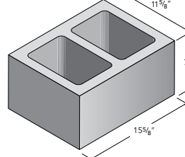
12x8x16 Spec-Brick
