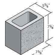
6x8x8 Standard
