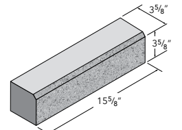
4x4x16 Solid Chamfer
