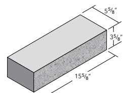
6x4x16 Solid
