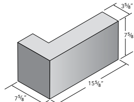
4x8x16 Spec-Brick L CNR
