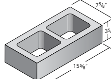
8x4x16 Spec-Brick
