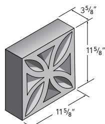
4x12x12 Viewlite 1
