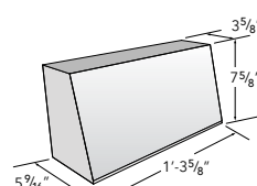
Abri Shingle
