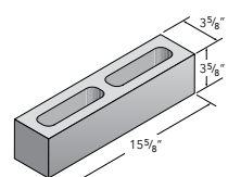
4x4x16 Spec-Brick
