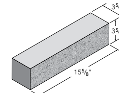
4x4x16 Solid
