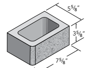
6x4x8 Single Bullnose
