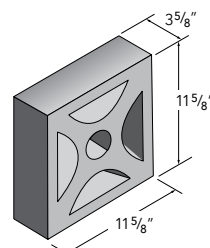
4x12x12 Viewlite 6
