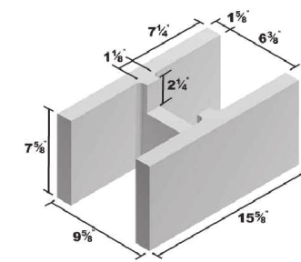
10x8x16 Double Open End Bond Beam
