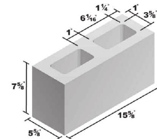
6x8x16 Standard
