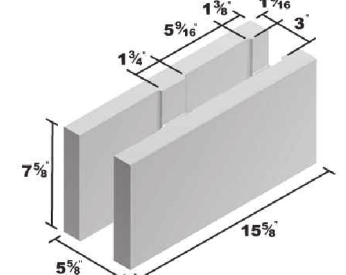
6x8x16 Open End Bond Beam
