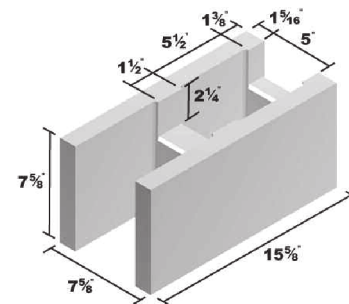
8x8x16 Open End Bond Beam
