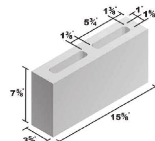
4x8x16 Partition
