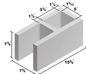
8x8x16 Open End Standard
