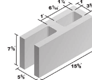
6x8x16 Open End Standard
