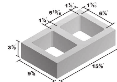
10x4x16 Standard
