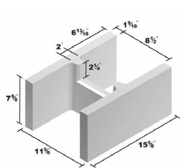
12x8x16 Double Open End Bond Beam
