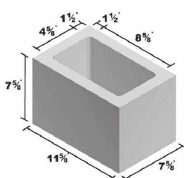
12x8x8 Half
