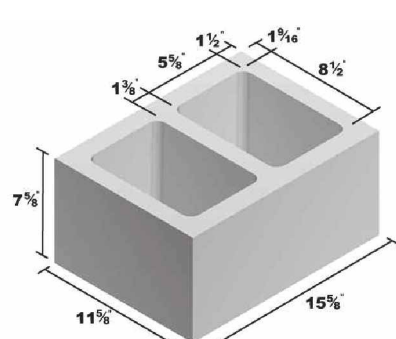
12x8x16 Standard
