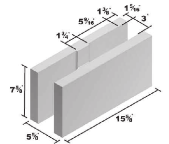
6x8x16 Double Open End Bond Beam
