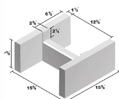
16x8x16 Double Open End Bond Beam
