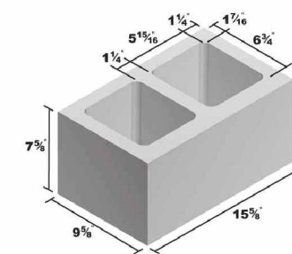
10x8x16 Standard
