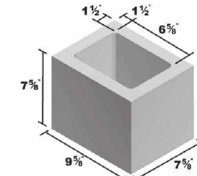
10x8x8 Half
