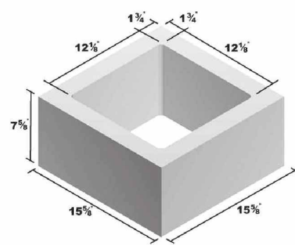
16x8x16 Column
