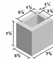
6x8x8 Half
