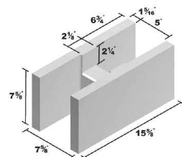
8x8x16 Double Open End Bond Beam
