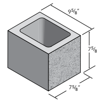
10X8X8 HALF — P | GF
