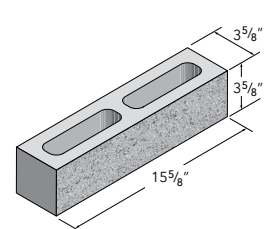
4X4X16 HALF HIGH
