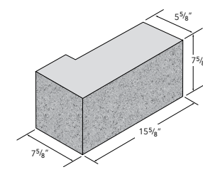
6X8X16 "L" CORNER SOLID
