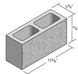
6X8X16 STANDARD
