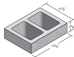
12X4X16 HALF HIGH — P | GF
