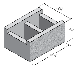
12X8X16 BOND BEAM — P | SF | GF
