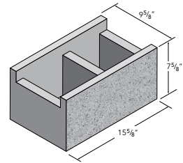
10X8X16 BOND BEAM — P | SF | GF
