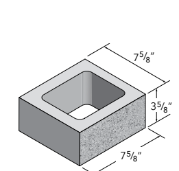
8X4X8 HALF HIGH HALF S1F
