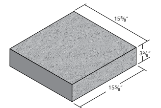
16X4X16 SOLID — P | GF
