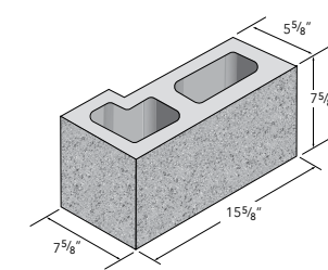
6X8X16 "L" CORNER
