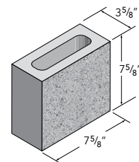
4X8X8 HALF
