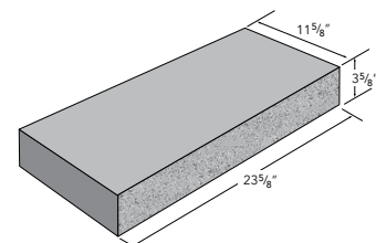
12X4X24 SOLID — P | GF
