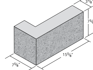
4X8X16 "L" CORNER SOLID
