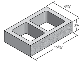
10X4X8 HALF HIGH — P | GF
