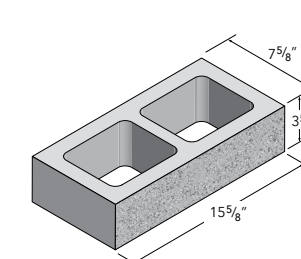
8X4X16 HALF HIGH
