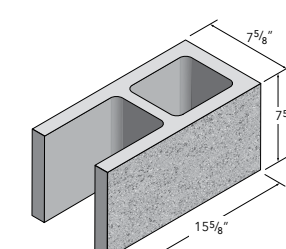
8X8X16 SINGLE OPEN END
