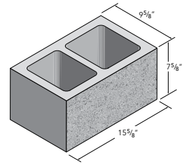
10X8X16 STANDARD — P | SF | GF
