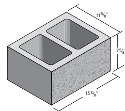
12X8X16 STANDARD — P | SF | GF
